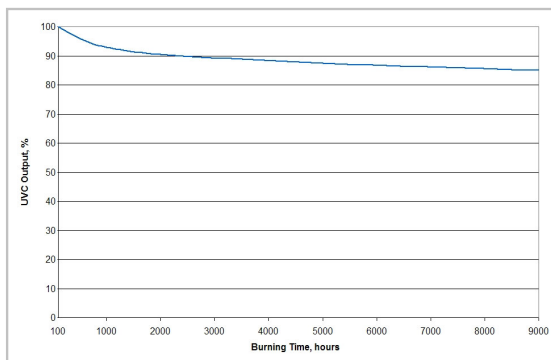
Maintenance Curve
