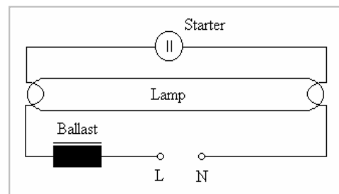
Wiring Diagram
