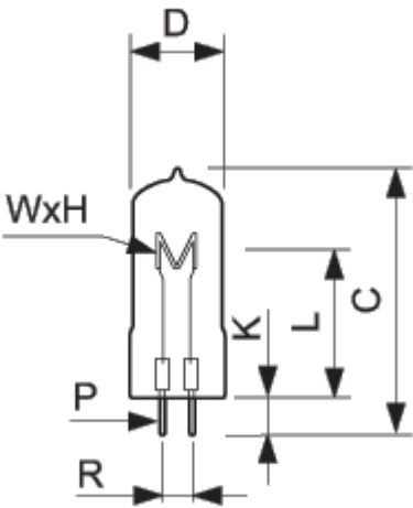
GX6.35 XHVPSE GX6.35
